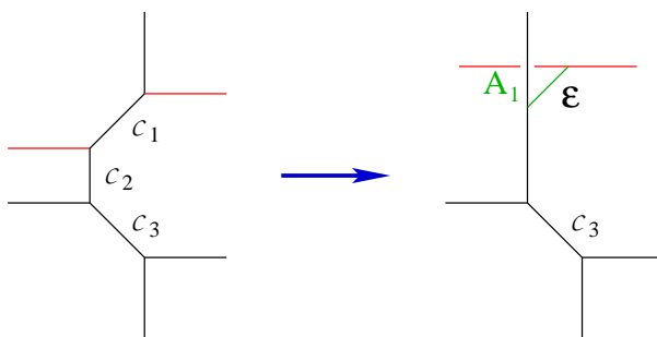
Figure 13: Deformation of the \mathbb{Z}_2 orbifold of the conifold given by (xy)(xy - \epsilon) = uv . The green segment represents an S^3 with volume proportional to its length.
